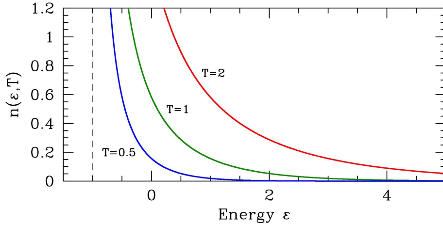
Figure 5.6: The Bose distribution n_{\epsilon}^B(T, \mu) = 1/[e^{(\epsilon-\mu)/k_B T} - 1] vs. \epsilon at fixed \mu = -1 ( k_B \equiv 1 ).
