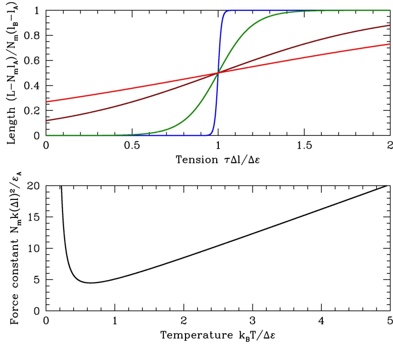
Figure 4.9: Upper panel: length L(\tau, T) for k_B T / \tilde{\varepsilon} = 0.01 (blue), 0.1 (green), 0.5 (dark red), and 1.0 (red). Bottom panel: dimensionless force constant N_m (\Delta l)^2 k / \varepsilon_A versus dimensionless temperature k_B T / \Delta \varepsilon .
