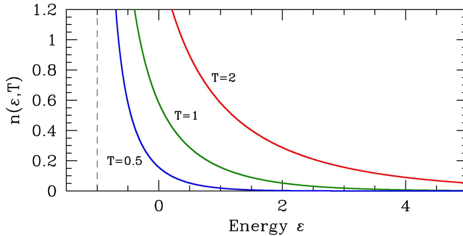
Figure 5.6: The Bose distribution n_{\varepsilon}^B(T, \mu) = 1/[e^{(\varepsilon-\mu)/k_B T} - 1] vs. \varepsilon at fixed \mu = -1 ( k_B \equiv 1 ).
