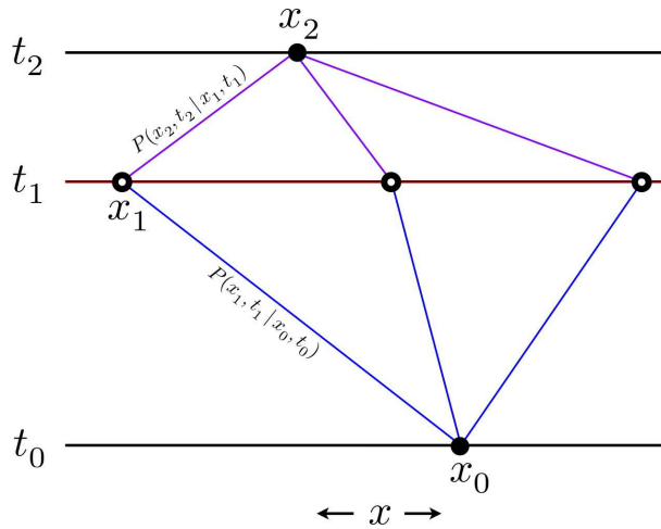
Figure 9.2: Interpretive sketch of the mathematics behind the Chapman-Kolmogorov equation.
