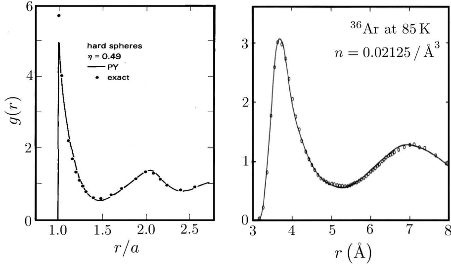
Figure 6.11: Pair distribution functions for hard spheres of diameter a at filling fraction \eta = \frac{\pi}{6}a^3n = 0.49 (left) and for liquid Argon at T = 85 K (right). Molecular dynamics data for hard spheres (points) is compared with the result of the Percus-Yevick approximation (see below in §??). Reproduced (without permission) from J.-P. Hansen and I. R. McDonald, Theory of Simple Liquids , fig 5.5. Experimental data on liquid argon are from the neutron scattering work of J. L. Yarnell et al. , Phys. Rev. A 7 , 2130 (1973). The data (points) are compared with molecular dynamics calculations by Verlet (1967) for a Lennard-Jones fluid.
