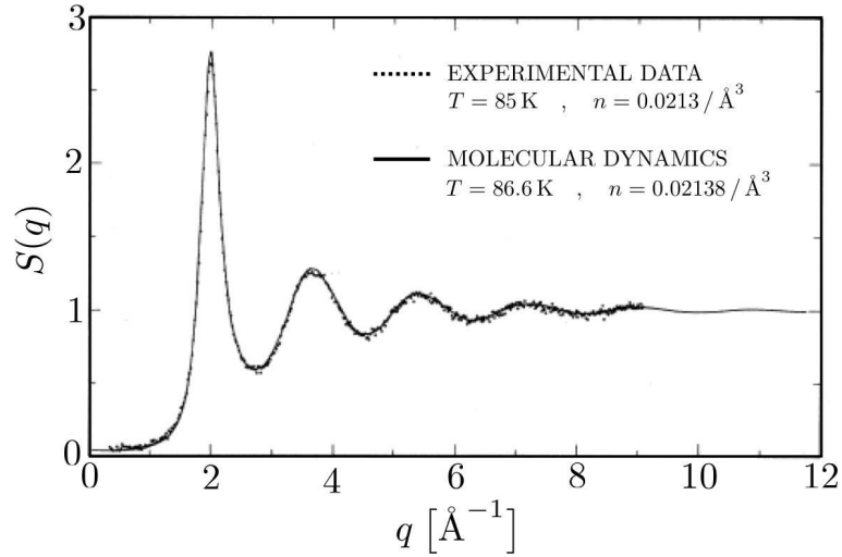
Figure 6.14: Comparison of the static structure factor of Argon as determined by neutron scattering work of J. L. Yarnell et al. , Phys. Rev. A 7, 2130 (1973) with molecular dynamics calculations by Verlet (1967) for a Lennard-Jones fluid.
