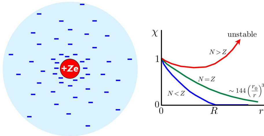
Figure 6.15: The Thomas-Fermi atom consists of a nuclear charge +Ze surrounded by N electrons distributed in a cloud. The electric potential \phi(\mathbf{r}) felt by any electron at position \mathbf{r} is screened by the electrons within this radius, resulting in a self-consistent potential \phi(\mathbf{r}) = \phi_0 + (Ze^2/r) \chi(r/r_0) .
