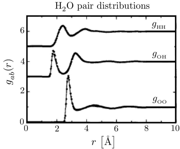
Figure 6.12: Monte Carlo pair distribution functions for liquid water. From A. K. Soper, Chem Phys. 202 , 295 (1996).
