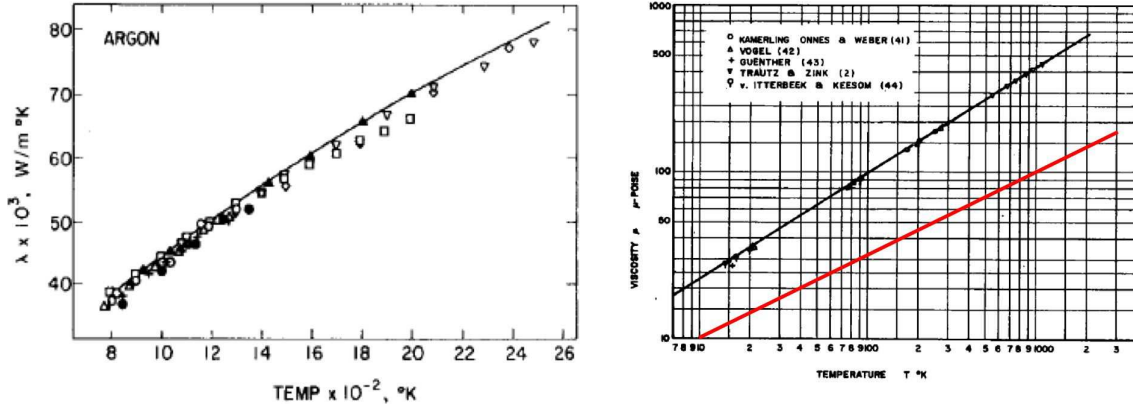
Figure 8.5: Left: thermal conductivity ( \lambda in figure) of Ar between T = 800 K and T = 2600 K. The best fit to a single power law \lambda = aT^b results in b = 0.651 . Source: G. S. Springer and E. W. Wingeier, J. Chem Phys. 59 , 1747 (1972). Right: log-log plot of shear viscosity ( \mu in figure) of He between T \approx 15 K and T \approx 1000 K. The red line has slope \frac{1}{2} . The slope of the data is approximately 0.633. Source: J. Kestin and W. Leidenfrost, Physica 25 , 537 (1959).
