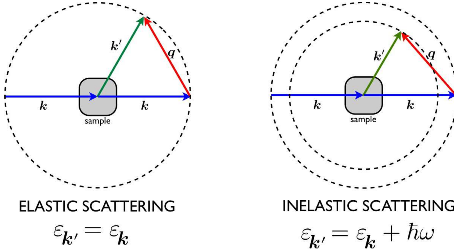
Figure 6.13: In a scattering experiment, a beam of particles interacts with a sample and the beam particles scatter off the sample particles. A momentum \hbar\mathbf{q} and energy \hbar\omega are transferred to the beam particle during such a collision. If \omega = 0 , the scattering is said to be elastic . For \omega \neq 0 , the scattering is inelastic .
