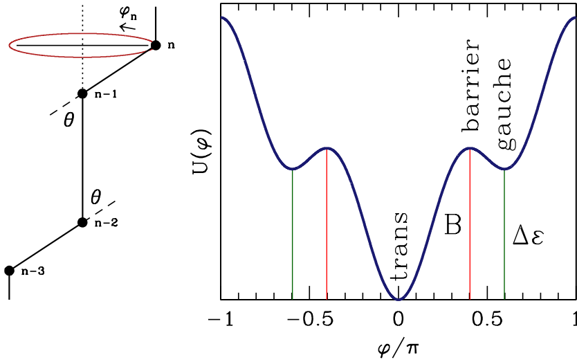
Figure 6.17: Left: trans and gauche orientations in carbon chains. Right: energy as a function of azimuthal angle \varphi . There are three low energy states: trans ( \varphi = 0 ) and gauche ( \varphi = \pm\varphi_0 ).
