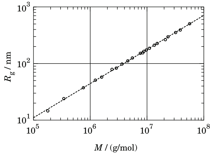
Figure 6.19: Radius of gyration R_g of polystyrene in a toluene and benzene solvent, plotted as a function of molecular weight of the polystyrene. The best fit corresponds to a power law R_g \propto M^\nu with \nu = 0.5936 . From J. Des Cloizeaux and G. Jannink, Polymers in Solution: Their Modeling and Structure (Oxford, 1990).
