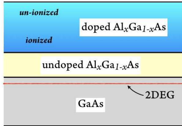
Figure 6.19: GaAs– \text{Al}_x\text{Ga}_{1-x}\text{As} heterojunction.
