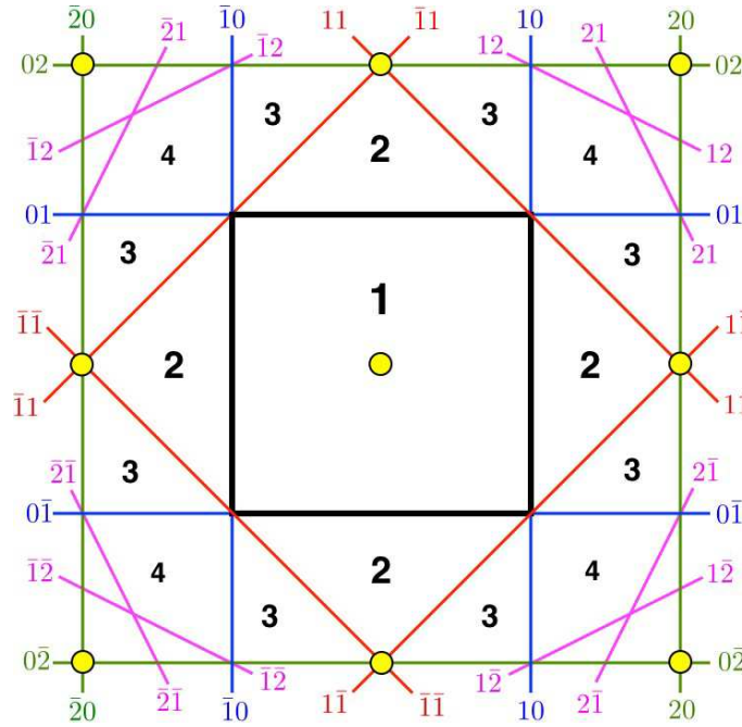
Figure 5.2: Extended zones and their folding for the square lattice. Reciprocal lattice points are shown as yellow dots. The central square, defined by the thick black line, is the first Brillouin zone. The colored lines denote bisectors of reciprocal lattice vectors G = n_1 b_1 + n_2 b_2 and are labeled by n_1 and n_2 . In general, a minimum of j - 1 such bisectors must be crossed in going from the j^{\text{th}} Brillouin zone to the first Brillouin zone., with j labeled in black. (Not all of the fourth zone is labeled.)
