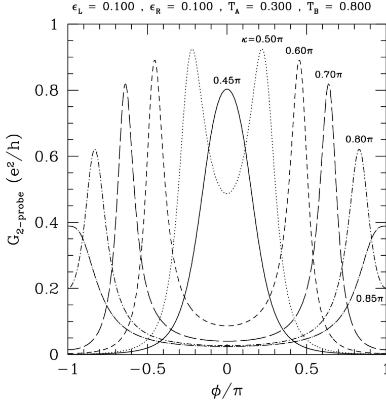
Figure 7.6: Two-probe conductance G(\phi, \kappa) of a model ring with two scatterers. The enclosed magnetic flux is \phi \hbar c/e , and \kappa = 2\pi kR (ring radius R ). G vs. \phi curves for various values of \kappa are shown.
