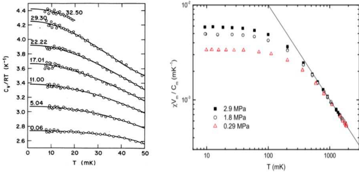
Figure 9.2: Left: c_V(T)/RT for normal ^3\text{He} . From D. S. Greywall, Phys. Rev. B 27 , 2747 (1983). Numbers give the sample pressures in bars at T = 0.1 K. Right: Normalized magnetic susceptibility \chi(T) v_0/C_m of normal ^3\text{He} , where v_0 is the molar volume and C_m \equiv \lim_{T \rightarrow \infty} T\chi(T) is the Curie constant. From V. Goudon et al. , J. Phys.: Conf. Ser. 150 , 032024 (2009).
