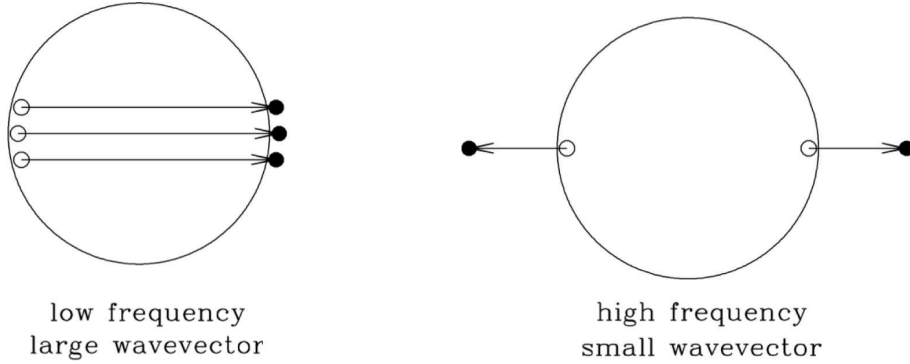
Figure 10.3: With multiple pair excitations, every part of (\mathbf{q}, \omega) space is accessible. However, these states do not couple to the ground state |\mathbf{G}\rangle through a single application of the density operator \hat{n}_{\mathbf{q}}^\dagger .
