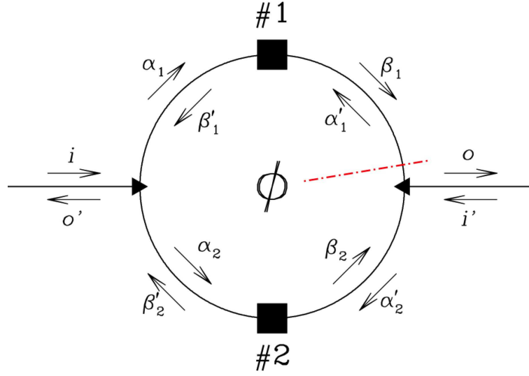
Figure 7.5: Scattering problem for a ring enclosing a flux \Phi . The square and triangular blocks represent scattering regions and are describes by 2 \times 2 and 3 \times 3 \mathcal{S} -matrices, respectively. The dot-dash line represents a cut across which the phase information due to the enclosed flux is accrued discontinuously.
