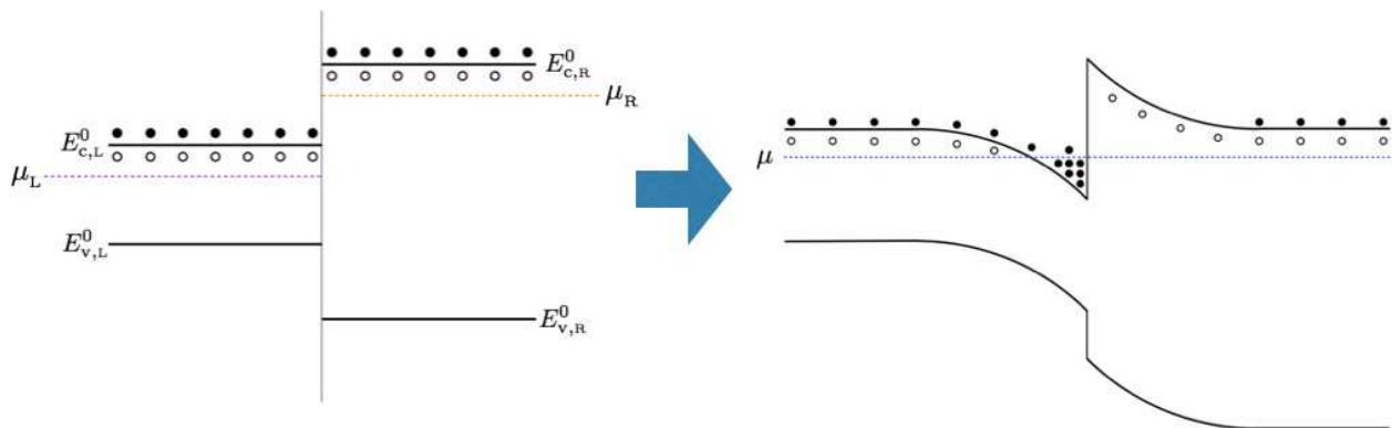
Figure 6.20: Accumulation layer formation in an n - n heterojunction.
