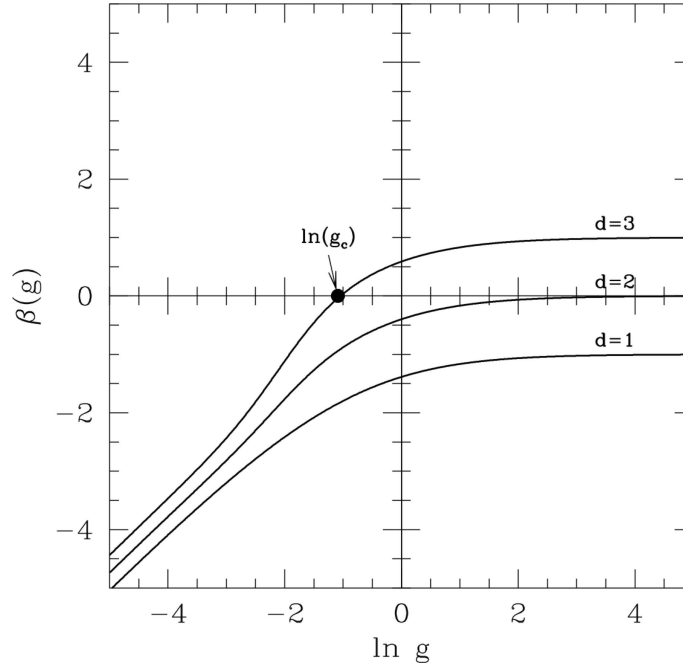
Figure 7.12: Sketch of the \beta -function for the localization problem for d = 1, 2, 3 . A critical point exists at g = g_c for the d = 3 case.
