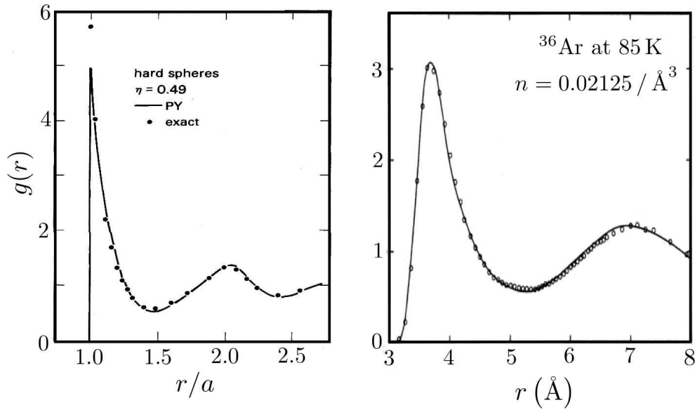
Figure 6.13: Pair distribution functions for hard spheres of diameter a at filling fraction \varphi = \frac{\pi}{6}a^3n = 0.49 (left) and for liquid Argon at T = 85 K (right). Molecular dynamics data for hard spheres (points) is compared with the result of the Percus-Yevick approximation (see below in §6.4.8). Reproduced (without permission) from J.-P. Hansen and I. R. McDonald, Theory of Simple Liquids , fig 5.5. Experimental data on liquid argon are from the neutron scattering work of J. L. Yarnell et al. , Phys. Rev. A 7, 2130 (1973). The data (points) are compared with molecular dynamics calculations by Verlet (1967) for a Lennard-Jones fluid.
