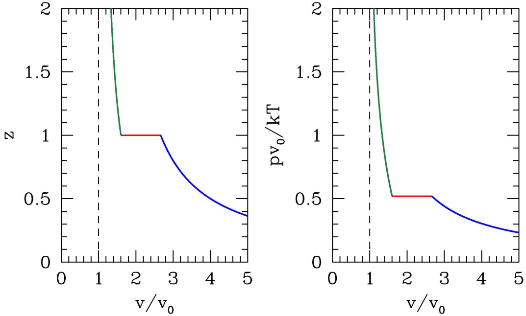
Figure 6.23: Fugacity z and pv_0/k_B T versus dimensionless specific volume v/v_0 for the example problem discussed in the text. The case r = 0.75 is shown.
