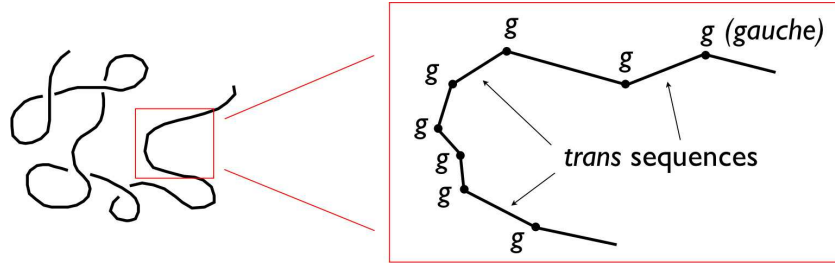
Figure 6.20: The polymer chain as a random coil.
