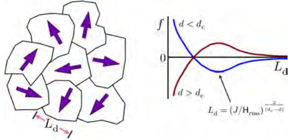
Figure 5: Left panel : Imry-Ma domains for an O(2) model. The arrows point in the direction of the local order parameter field \langle \hat{\mathcal{N}}(\mathbf{r}) \rangle . Right panel : free energy density as a function of domain size L_d . Note L_d > a always.
