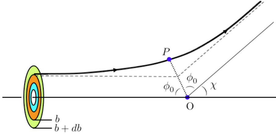
Figure 8.6: Scattering in the CM frame. O is the force center and P is the point of periastris. The impact parameter is b , and \chi is the scattering angle. \phi_0 is the angle through which the relative coordinate moves between periastris and infinity.
