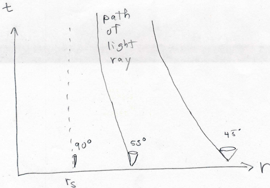
Light comes near black hole,
