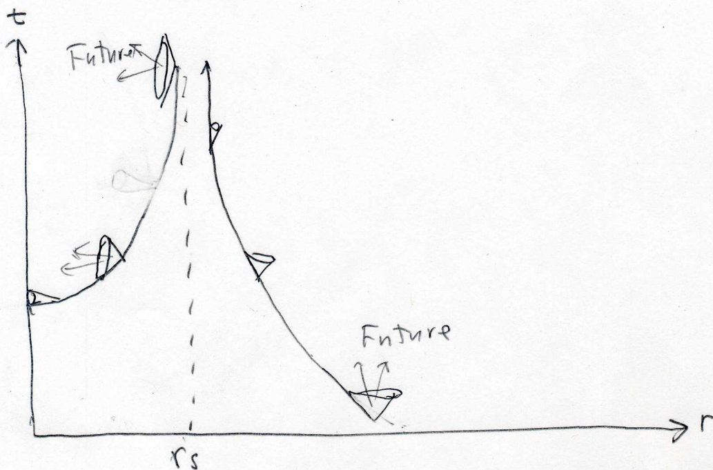
Light comes inside black hole
