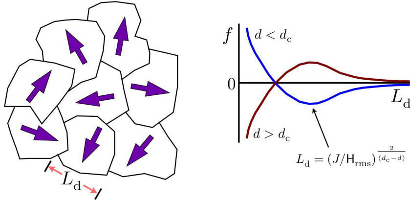
Figure 7.23: Left panel : Imry-Ma domains for an O(2) model. The arrows point in the direction of the local order parameter field \langle \hat{\mathcal{O}}(\mathbf{r}) \rangle . Right panel : free energy density as a function of domain size L_d . Keep in mind that the minimum possible value for L_d is the lattice spacing a .
