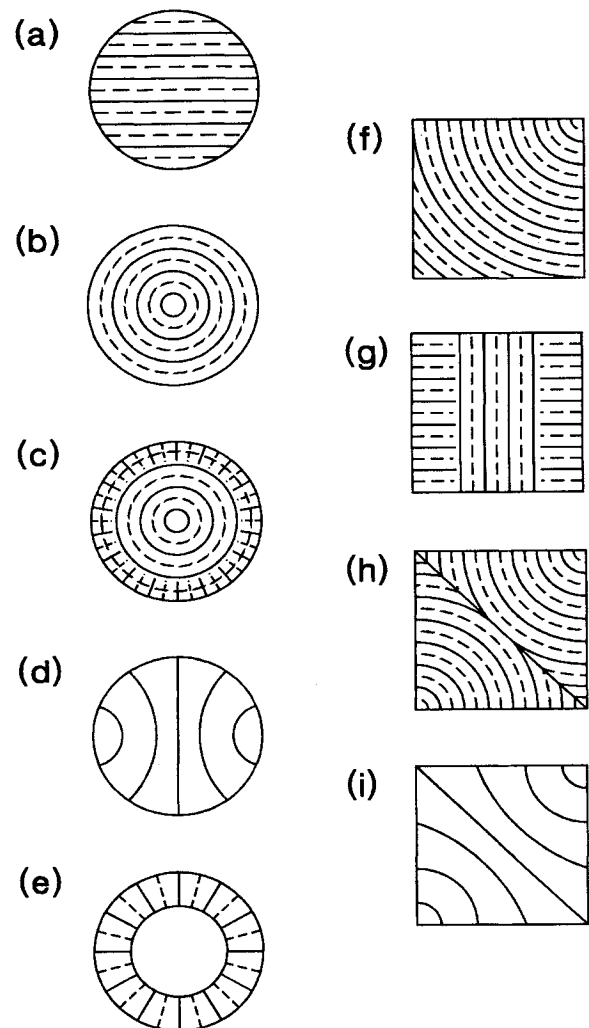
FIG. 21. Schematic of possible patterns in Rayleigh-Bénard convection and other type I_1 systems. Solid and dashed lines represent roll boundaries (e.g. upflow and downflow, respectively). In (d) and (i) only a coarse grained representation of the roll boundary directions is shown, and there are many dislocations on a finer scale not shown, which permit the large scale distortions.
