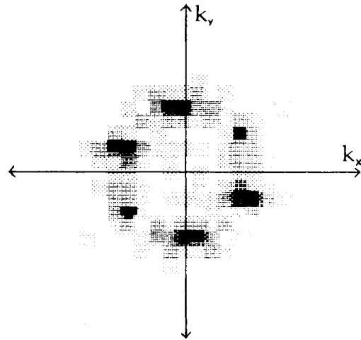
FIG. 51. Hexagon pattern in modulated convection. (a) Shadowgraph image of a hexagonal convection pattern achieved with modulation parameters \omega = 1.5 , \delta = 1.97 , and \varepsilon_0 = 0.20 in Eq. (8.101). The bright regions show downflow at the center of the hexagons, while the dark regions show upflow along their outer boundaries. (b) Low-wave-vector portion of the Fourier transform of the image in (a), demonstrating the sixfold symmetry of the pattern. (From Meyer et al. , 1988.)
