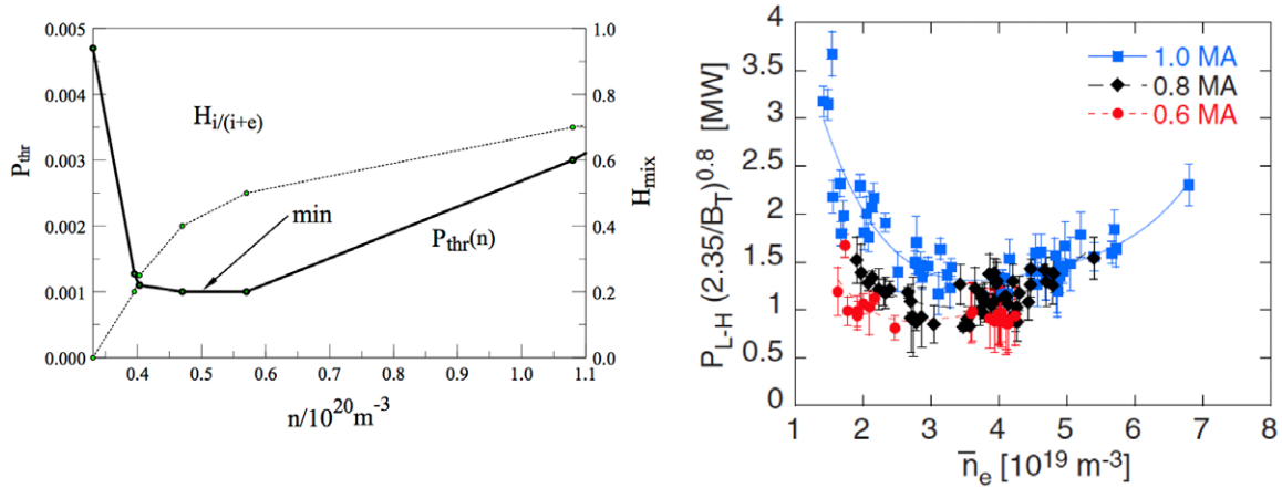
Figure 9. Left: (a) Variation of P_{\text{th}}(n) with density for the given heating mix evolution H_{ii+e}(n) . Figure adapted from [38]. Right: (b) variation of P_{\text{th}}(n) in AUG, showing non-monotonic evolution with plasma density. Panel (b) adapted from [37].
