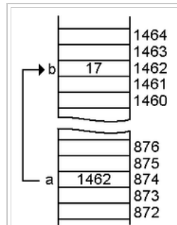
Pointer a pointing variable b . Note that b stores number, whereas a stores address of b in memory (1462)
