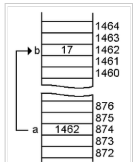
Pointer a pointing variable b . Note that b stores number, whereas a stores address of b in memory (1462)
