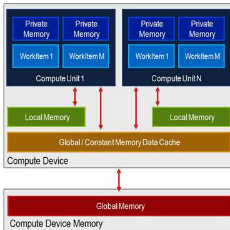
Figure 8: OpenCL Memory Hierarchy. Figure taken from[30].
