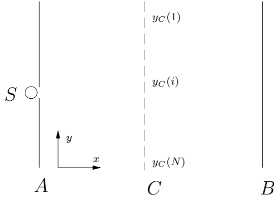
Figure 2: Set-up for thought experiment with N slits
