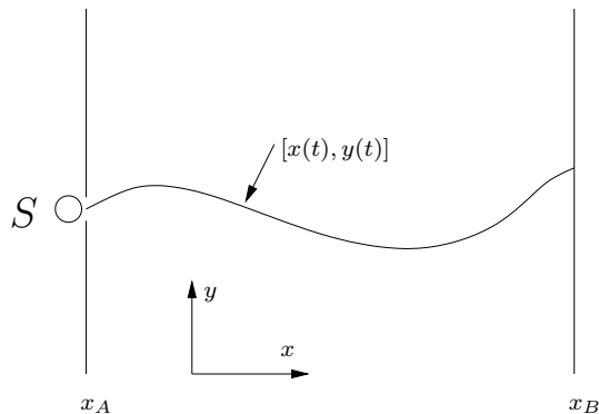
Figure 3: A complete path between A and B
