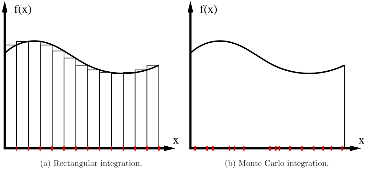
Figure 5: Comparing rectangular integration with simple Monte Carlo integration.
