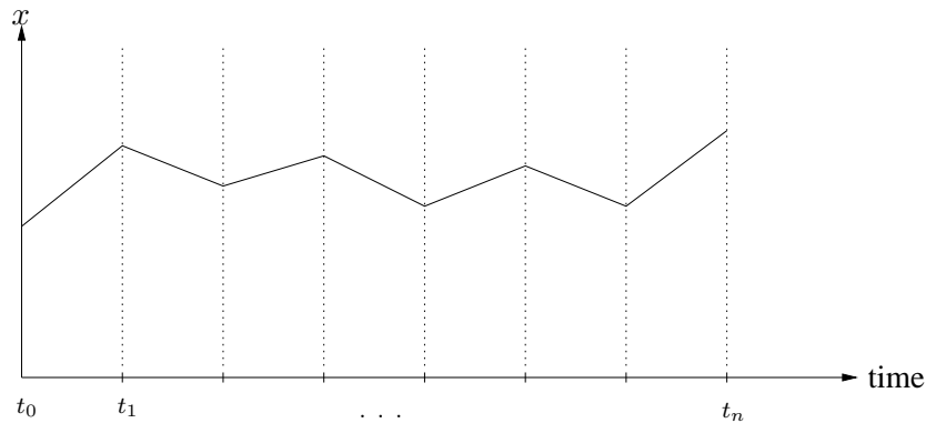
Figure 4: A discrete path
