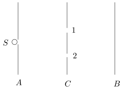
Figure 1: Double-slit experiment set-up
