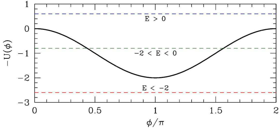
Figure 8.9: The inverted potential -U(\phi) = \cos \phi - 1 for the sine-Gordon problem.
