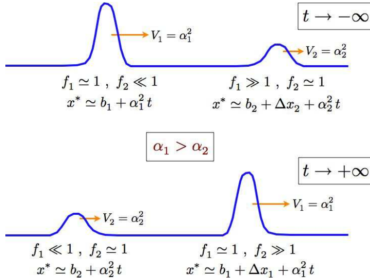
Figure 8.5: Early and late time configuration of the two soliton solution to the KdV equation.
