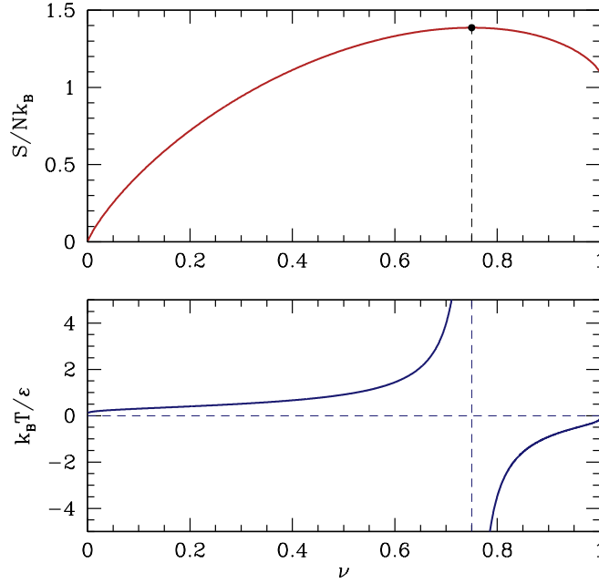
Figure 1: Bottom: dimensionless temperature \theta(\nu) \equiv k_B T/\varepsilon versus dimensionless energy density \nu = E/N\varepsilon for problem 1, shown here for g = 3 . Note that T \rightarrow \mp\infty for \nu \rightarrow \nu^* \pm 0^+ , where \nu^* = g/(g+1) is the energy density at which the entropy is maximum. Top: dimensionless entropy s(\nu) \equiv S/Nk_B versus dimensionless energy density \nu . Note the maximum at \nu^* = g/(g+1) , where g is the degeneracy of the excited level.
