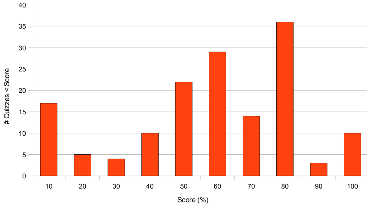
Quiz 2 Histogram
