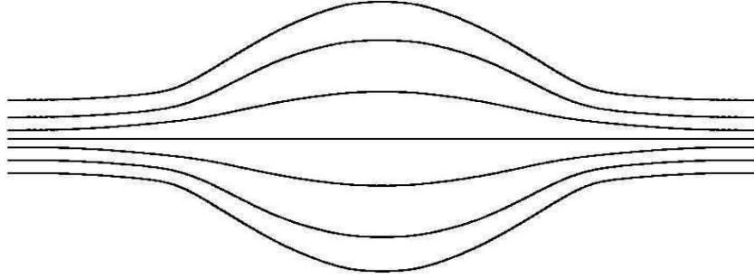
Figure 5.7: B field lines in a magnetic bottle.
