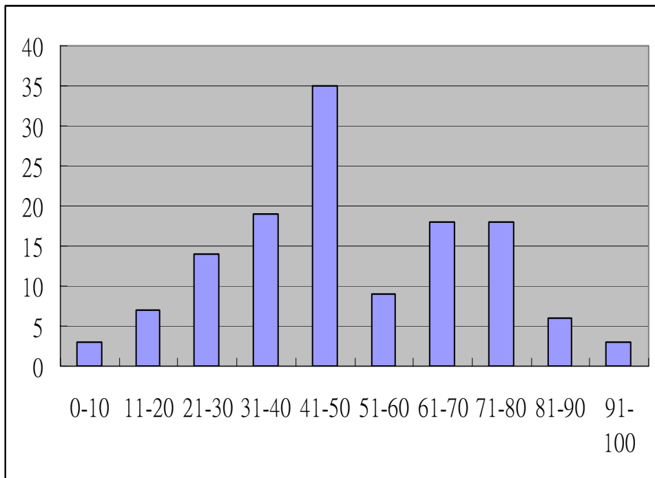
Curriculum Histogram (lowest one dropped)
